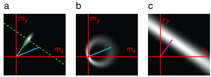
Figure B1. Derivation of the likelihood function. (a) Gaussian probability distribution of normal velocity measurements (grayscale), p(\vec{m} | \theta, \vec{v}) , for a grating with normal velocity specified by the green vector, but moving at physical velocity specified by the blue vector. The constraint line (dashed green) of all translational velocities consistent with the normal velocity of that grating is also shown. (b) The distribution of normal velocity measurements (grayscale), p(\vec{m} | \vec{v}) , for an arbitrary spatial pattern moving with the specified physical velocity (blue vector). This is computed by integrating over all directions, \theta , as in Equation B3. (c) The likelihood, a function of \vec{v} , obtained by evaluating p(\vec{m} | \vec{v}) for a particular normal velocity measurement \vec{m} (magenta vector) drawn from the distribution in (a).
