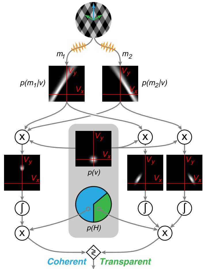
Figure 2. Illustration of the Bayesian observer model, responding to a single presentation of a plaid. In the encoding stage (not shown), an observer makes noisy measurements \{\bar{m}_1, \bar{m}_2\} of the normal velocities of the two gratings. In the decoding stage, the observer forms separate likelihood functions for the two component motions based on their associated measurements. These are combined with prior preferences (internal to the observer's visual system) in order to arrive at a percept. Internal preferences are contained within the gray region and include a prior distribution over velocity, p(\bar{v}) , and a prior probability of coherent motion, p(H) . For the coherent motion percept, both likelihoods are multiplied together with the velocity prior, and this posterior distribution is then integrated (left). For the transparent percept, each likelihood is individually multiplied by the velocity prior and integrated (right). The resulting scalar values are then multiplied by the internal prior for coherence/transparency, yielding posterior probabilities for each of the percepts. Finally, these are compared, and the larger one is selected as the percept.
