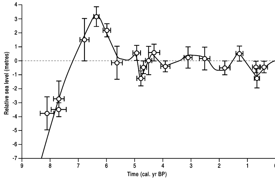
Fig. 6. Holocene sea-level fluctuations inferred from sea-level index points from the southern Langebaan Lagoon salt marsh, South Africa. Horizontal error bars refer to analytical uncertainty in radiocarbon age calibration ( 2\sigma range), and vertical error bars refer to uncertainty in sea level predictions derived from organic matter and shell material indicators (modified from Compton, 2001).
