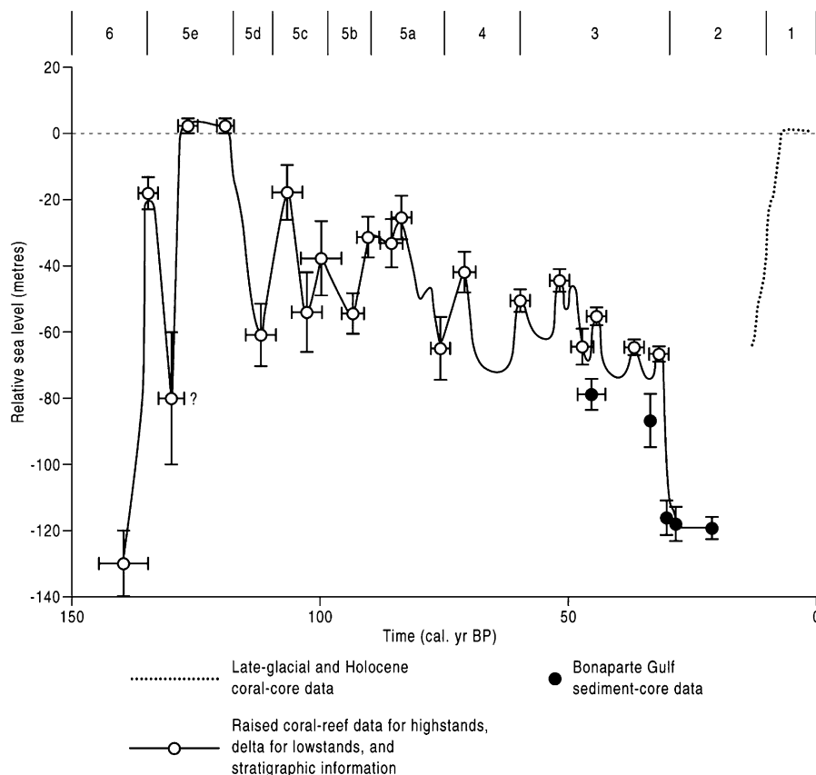
Fig. 1. The relative sea-level curve for the last glacial cycle for Huon Peninsula (Lambeck and Chappell, 2001) supplemented with observations from Bonaparte Gulf, Australia (Yokoyama et al., 2000). Error bars define the upper and lower limits (modified from Lambeck et al., 2002).
