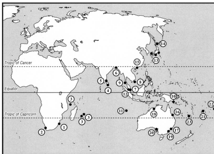
Fig. 5. Location of sea-level reconstructions in the Indo-Pacific region. Numbers refer to locations in Table 1.
