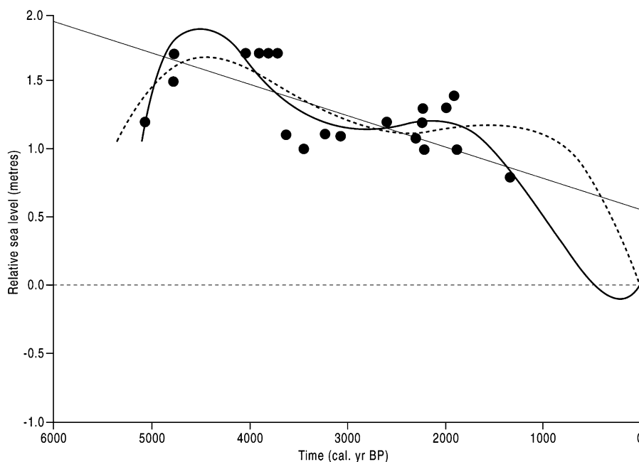
Fig. 8. A summary of linear and oscillating regression models from sea-level index points created using fixed biological indicators from SE Australia for the past 5000 years. Dotted line—4th order polynomial ( r^2 = 0.69 ), smooth line—5th order polynomial ( r^2 = 0.78 ) (after Baker et al., 2001).
