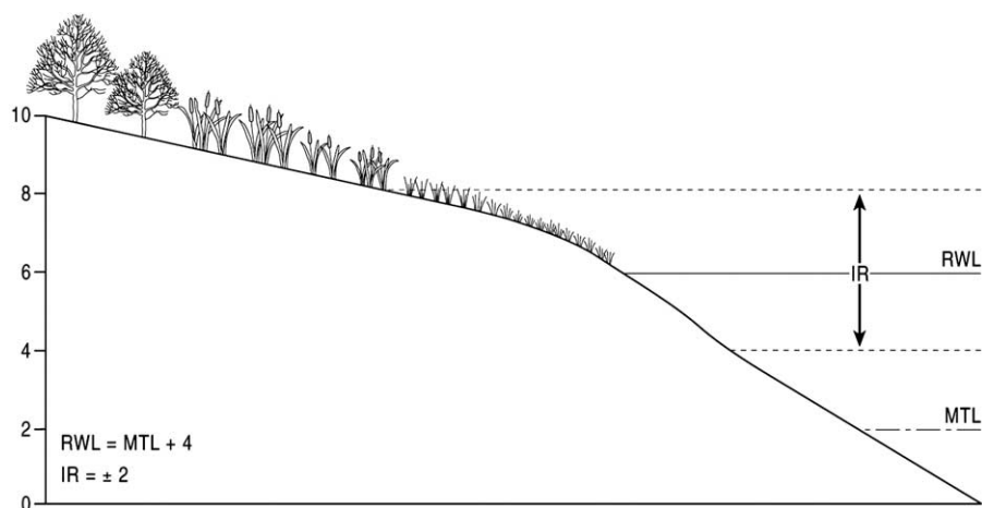
Fig. 3. Schematic diagram of the Indicative Meaning illustrating the how the Indicative Range (IR) and Reference Water Level (RWL) are derived from Mean Tide Level (MTL) (not drawn to scale).
