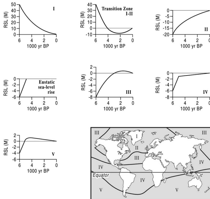
Fig. 2. Sea-level zones and typical relative sea-level curves deduced for each zone by Clark et al. (1978) under the assumption that no eustatic change has occurred since 5 ka BP.
