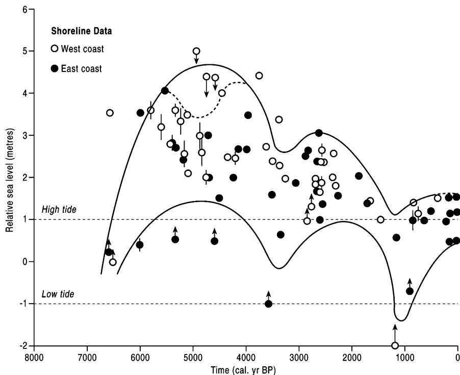
Fig. 7. Holocene sea-level envelope for Peninsula Malaysia (modified from Tija, 1996). Data points with arrows indicate directional (limiting) index points. Some index points have vertical error bars, where the vertical range of the sea-level indicator is understood. No age errors are considered, radiocarbon ages are plotted. The boundaries of the envelope are drawn midway between the extreme data points and the neighbouring points within the envelope (Tija, 1996).
