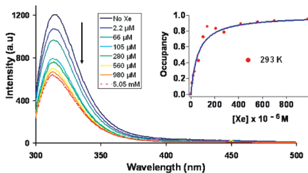
Figure 1. Fluorescence quenching of 1 (15 \mu\text{M} ) by Xe in 1 mM, pH 7.2 phosphate buffer, 293 K. Inset: Curve fits for a single-site binding model.
