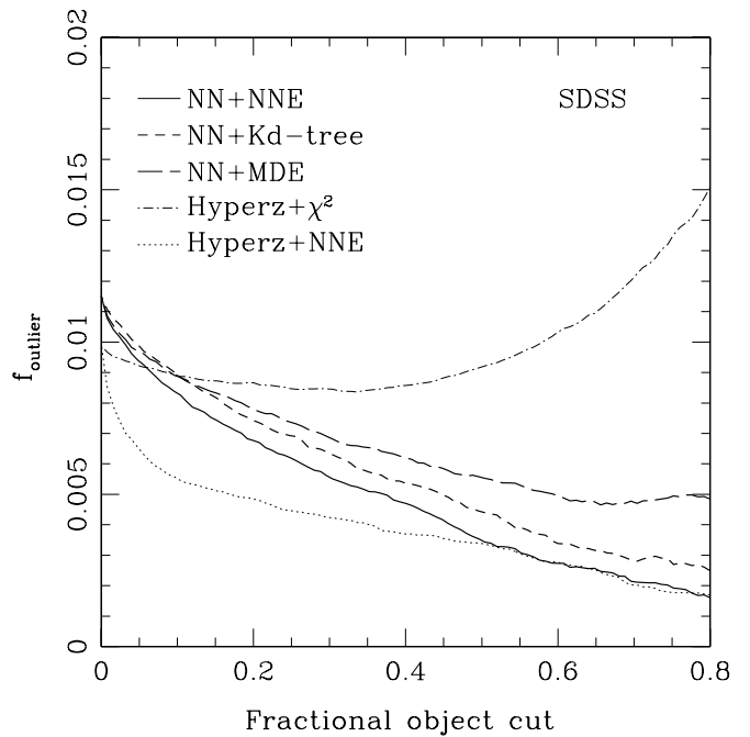
FIG. 10.—Same as Fig. 9, but for the SDSS catalog. Note that the scatter and the outlier fraction do not improve when the catalog is cut using the \chi^2 errors.
