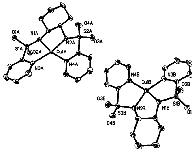
Figure 2. Structure of 2res . Important distances (Å) and angles (deg): Cu(1A)–N(1A) = 1.971(8), Cu(1A)–N(2A) = 1.966(7), Cu(1A)–N(3A) = 2.080(8), Cu(1A)–N(4A) = 2.022(8), Cu(1A)–O(1A') = 2.410(8), Cu(1B)–N(1B) = 1.960(8), Cu(1B)–N(2B) = 1.947(7), Cu(1B)–N(3B) = 2.022(6), Cu(1B)–N(4B) = 2.033(9), N(1A)–Cu(1A)–N(2A) = 83.5(3), N(2A)–Cu(1A)–N(3A) = 167.4(3), N(3A)–Cu(1A)–N(4A) = 107.7(3), N(1A)–Cu(1A)–N(4A) = 167.7(3), N(1A)–Cu(1A)–N(3A) = 84.1(3), N(2A)–Cu(1A)–N(4A) = 85.5(3), N(1B)–Cu(1B)–N(2B) = 83.5(3), N(2B)–Cu(1B)–N(3B) = 156.3(3), N(3B)–Cu(1B)–N(4B) = 106.7(3), N(1B)–Cu(1B)–N(4B) = 160.8(3), N(1B)–Cu(1B)–N(3B) = 88.3(3), N(2B)–Cu(1B)–N(4B) = 86.8(3).
