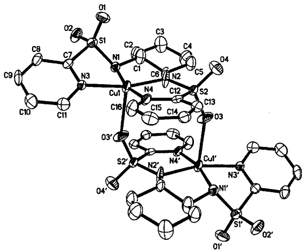
Figure 1. Structure of dimeric 2rac . Important distances (Å) and angles (deg): Cu(1)–N(1) = 1.985(6), Cu(1)–N(2) = 1.951(6), Cu(1)–N(3) = 2.026(6), Cu(1)–N(4) = 2.043(6), Cu(1)–O(3') = 2.328(6), S(1)–O(1) = 1.444(6), S(1)–O(2) = 1.436(6), S(2)–O(3) = 1.451(6), S(2)–O(4) = 1.428(6), N(1)–Cu(1)–N(2) = 83.7(3), N(2)–Cu(1)–N(3) = 165.7(3), N(3)–Cu(1)–N(4) = 103.2(2), N(1)–Cu(1)–N(4) = 165.9(2).
