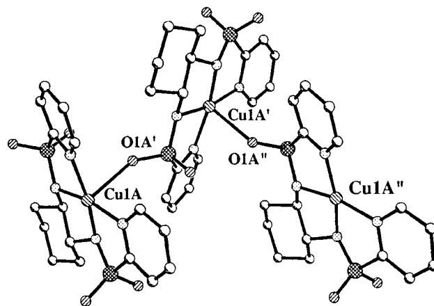
Figure 3. Polymeric structure of 2res molecule A. Cu(1A)–O(1A') = 2.410(8).
