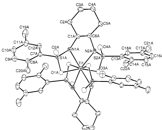
Figure 6. ORTEP drawing of C 2 -8homo is shown. The atoms are shown at 30% probability. Bond lengths and bond angles are shown in Tables 1 and 2.
