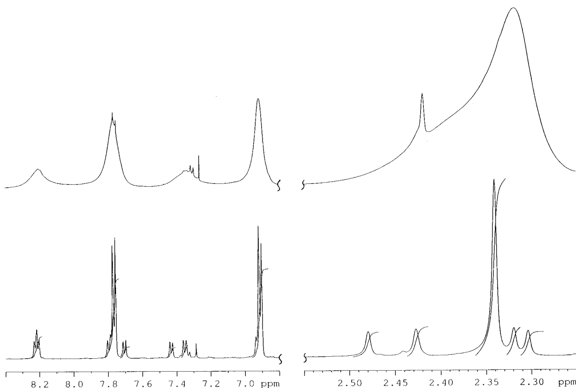
Figure 2. ^1\text{H} NMR spectra of \text{C}_2\text{-6homo}/\text{C}_s\text{-6homo} equilibrium in \text{CDCl}_3 at 23\text{ }^\circ\text{C} (top) and at -15\text{ }^\circ\text{C} (bottom).
