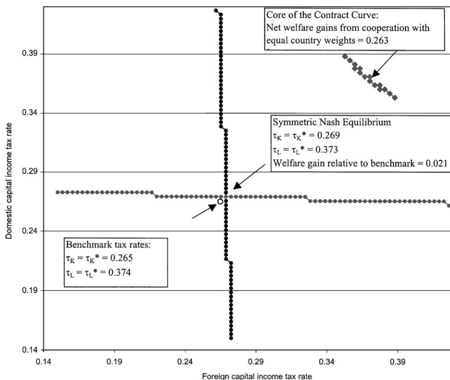
Fig. 6. Reaction curves for symmetric tax competition game over capital income tax rates with adjustment in labor income tax rates.
