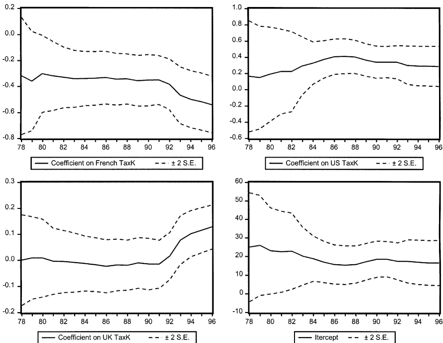
Fig. 5. Recursive estimates of coefficients in OLS regression of French investment rate (sample period: 1970–1996, adj. R^2 = 0.733 ).
