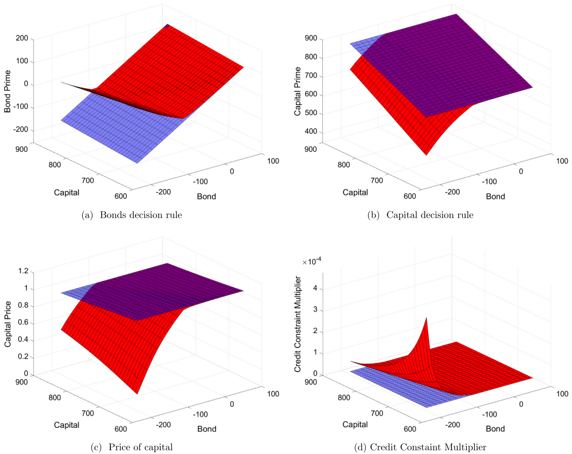
Note: All plots show solutions obtained with the FiPlt method. Surface plots in red (blue) are for the SS (RBC) model.
