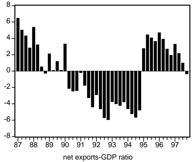
Figure 1. Mexico's Sudden Stop (percent changes with respect to the same quarter of the previous year)
