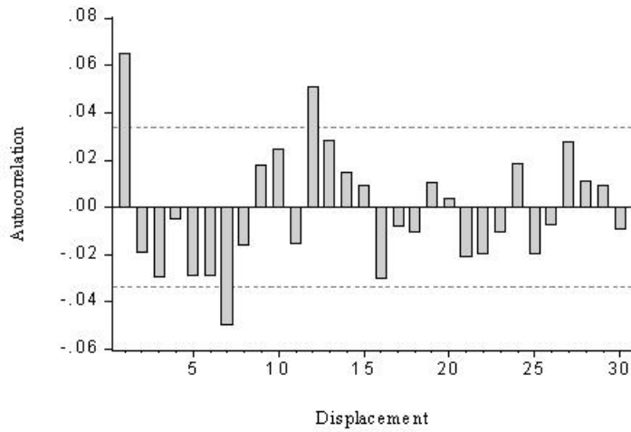
Figure 10.2: Correlogram of Daily NYSE Returns.
