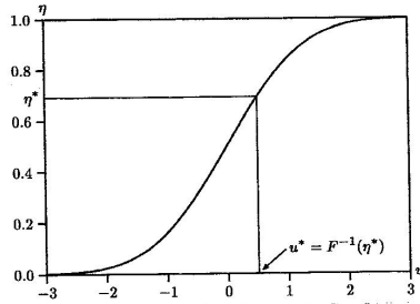
Figure 5.2: Transforming from U(0,1) to f (from Davidson and MacKinnon, 1993)
