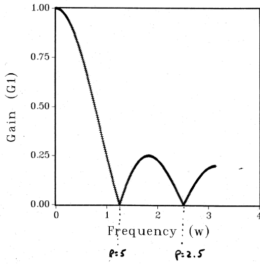
Figure 2.3: Gain of Kuznets' Filter 1
