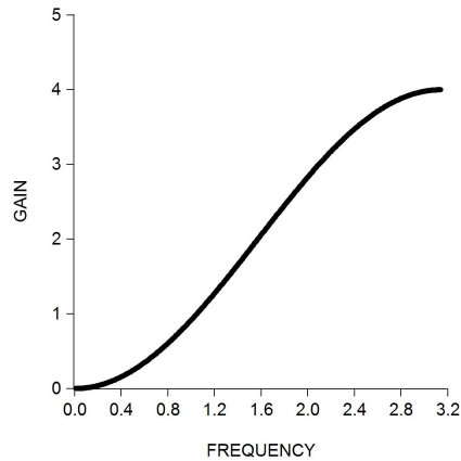
Figure 2.2: Gain of Differencing Filter 1 - L
