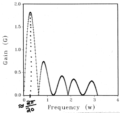
Figure 2.5: Composite Gain of Kuznets' two Filters
