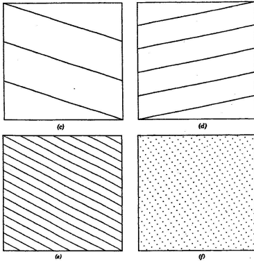
Figure 5.1: Ripley's "Horror" Plots of pairs of (U_{i+1}, U_i) for Various Congruential Generators Modulo 2048 (from Ripley, 1987)
