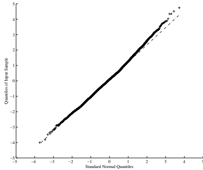
Figure 10.18: QQ Plot of S&P500 Returns Standardized by Realized Volatilities. We show quantiles of daily S&P500 returns standardized by AvgRV against the corresponding quantiles of a standard normal distribution. The sample period is January 2, 1990 through December 31, 2010. The units on each axis are standard deviations.
