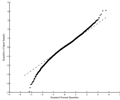
Figure 10.17: QQ Plot of S&P500 Returns Standardized by NGARCH Volatilities. We show quantiles of daily S&P500 returns standardized by the dynamic volatility from a NGARCH model against the corresponding quantiles of a standard normal distribution. The sample period is January 2, 1990 through December 31, 2010. The units on each axis are standard deviations.
