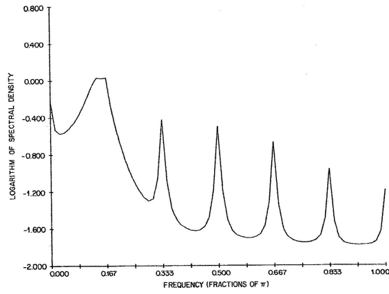
Figure 2.1: Granger's Typical Spectral Shape of an Economic Variable
