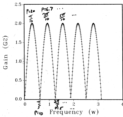
Figure 2.4: Gain of Kuznets' Filter 2
