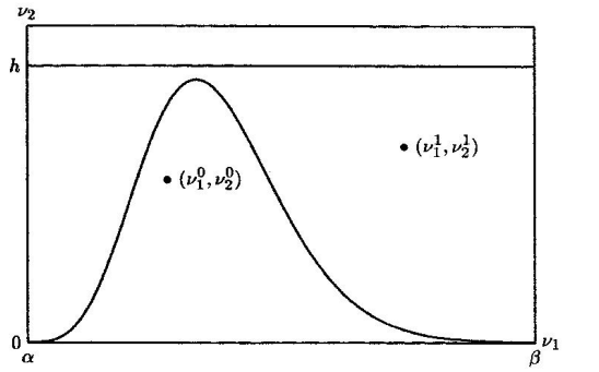
Figure 5.3: Naive Accept-Reject Method
