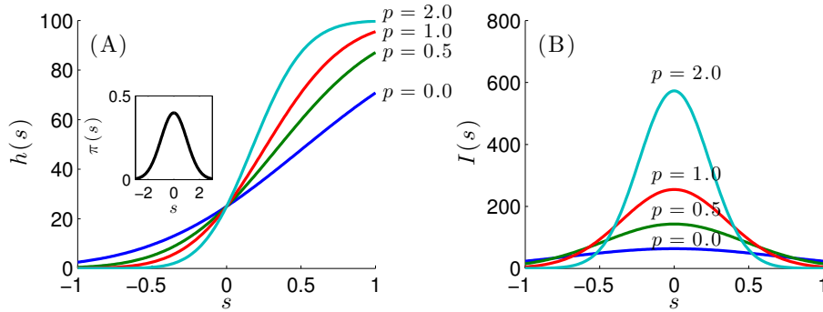
Figure 2: (A) The f_p -optimal tuning curve for standard Gaussian prior (inset figure) with various values of p . When p = 2 the f_2 -optimal tuning curve minimizes the squared loss ( discrimax ) and when p = 0 the f_0 -optimal maximizes the mutual information ( infomax ). (B) The Fisher Information \mathcal{I}(s) for f_p -optimal tuning curve with various values of p .
