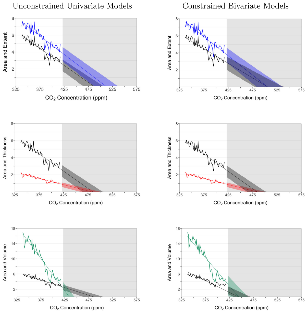
Fig. 2. September Arctic sea-ice indicators: Estimated linear carbon trends in ice-carbon space under SSP3 7.0. Notes: Each panel displays a pair of sea-ice indicators graphed against CO 2 C (atmospheric CO 2 concentration, measured in ppm). We show extent in blue (measured in 10 6 km 2 ), area in black (measured in 10 6 km 2 ), thickness in red (measured in m), and volume in green (measured in 10 3 km 3 ). In the univariate column, we show linear carbon-trend fits and projections based on Eq. (3). In the bivariate column, we show linear carbon-trend regression fits and forecasts constrained to reach zero simultaneously, based on Eq. (4). The historical sample period (unshaded) is 1979–2021, and the projection intervals obtained by simulation have 90% coverage. See Appendix B for details.
