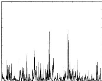
Factor-GARCH Series 1 Squared
