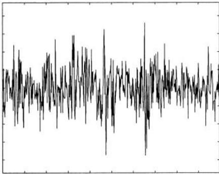
Factor-GARCH Series 1
