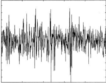
GARCH(1,1) Realization
