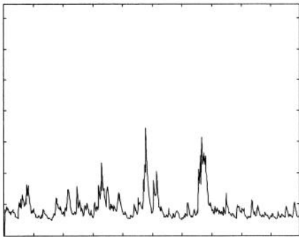
Conditional Variance of Series 1
