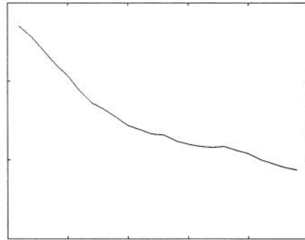
Sample Autocorrelation Function
