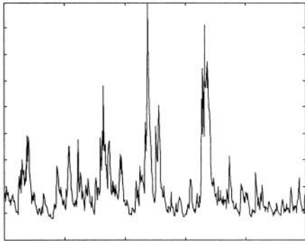
Conditional Variance
