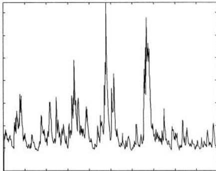
Conditional Variance of Series 2
