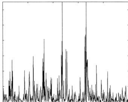
Squared GARCH(1,1) Realization
