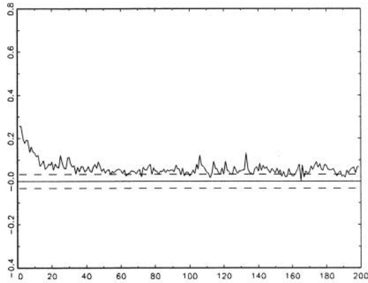
Autocorrelation Function-S&P \epsilon^2 - Jan 28 to Dec 40
