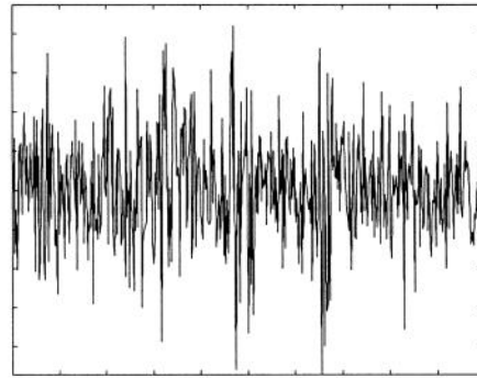
Factor-GARCH Series 2
