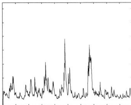
Conditional Covariance
