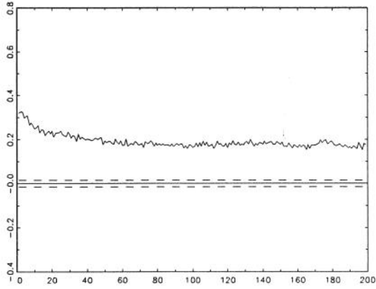
Autocorrelation Function-S&P |\epsilon| - Jan 28 to May 90
