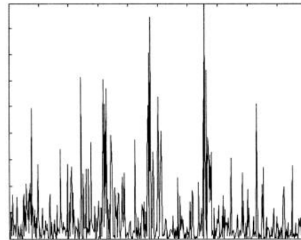
Factor-GARCH Series 2 Squared
