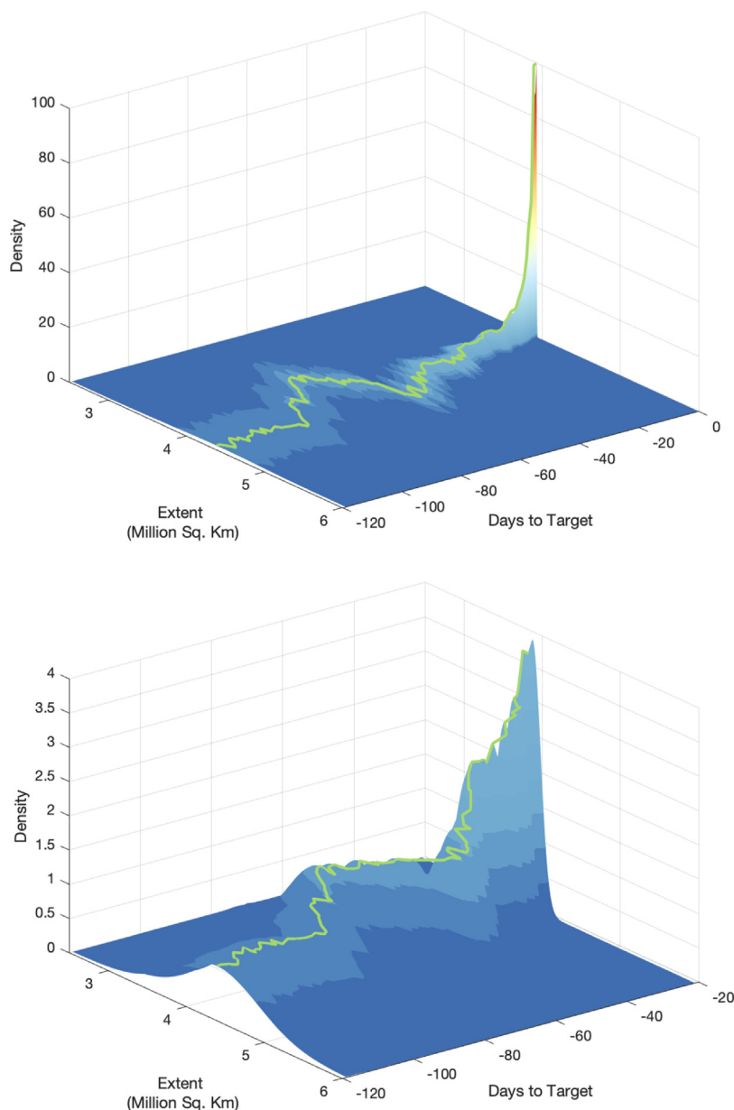
Fig. 2. Arctic sea ice extent: day-by-day predictive densities for September 2020. Notes: We show the sequence of 120 day-by-day predictive densities for September 2020 average daily Arctic sea ice extent as September 30 is approached. The horizontal axis represents the number of days until the end of September, and the green line is the point forecast (the mean of the predictive density). Top: we show the entire [-120, 0] sequence. Bottom: we zoom in on [-120, -20] , to enhance visualization detail.
