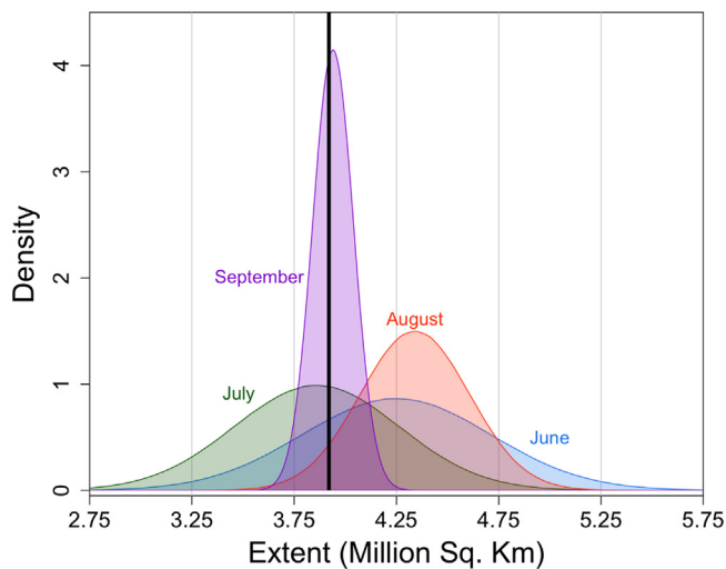
Fig. 1. Arctic sea ice extent: four predictive densities for September 2020. Notes: We show four predictive densities for September 2020 Arctic sea ice extent (monthly average of daily values). Forecasts are made on the 10th of the month. The vertical black line is the realized September value. See text for details.
