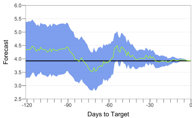
Fig. 3. Arctic sea ice extent: day-by-day predictive intervals for September 2020. Notes: We show the sequence of day-by-day prediction intervals for September 2020 average daily Arctic sea ice extent as September 30 is approached. The horizontal axis represents the number of days until the end of September, the green line is the point forecast (the midpoint of the prediction interval), and the shaded area is the \pm 2 standard error band. The horizontal black line is the realized September value.
