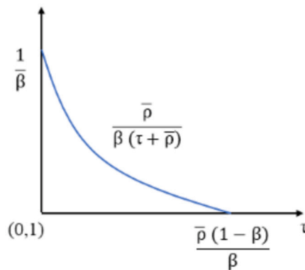
Fig. 7. Optimal policy.
