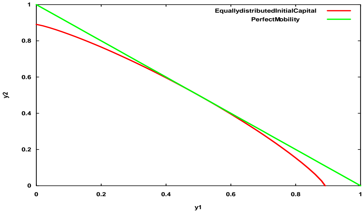
Figure 3: Capital Mobility, M(x, y_1, y_2) = x^{-\gamma} y_1^{1+\gamma} + (1 - x)^{-\gamma} y_2^{1+\gamma} - 1 , x = 0.5 , \gamma = 0.2
